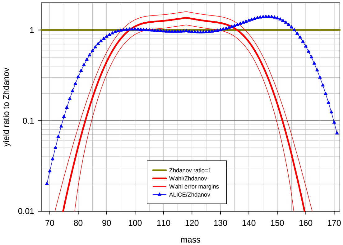
Benchmark B: ^{241}\text{Am} at 160 MeV, pre-neutron emission yield ratio to Zhdanov's data
